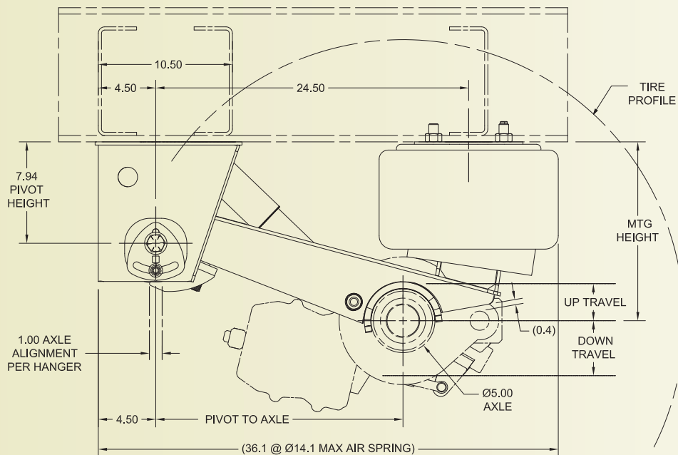
14 INCH MOUNTING HEIGHT SHOWN
