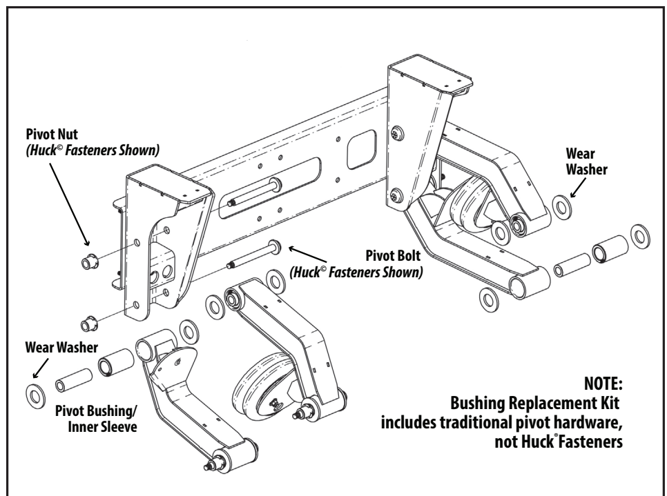
Figure 2. The bushing replacement kit with hardware includes traditional hardware to replace the Huck® Fasteners used for initial assembly.
