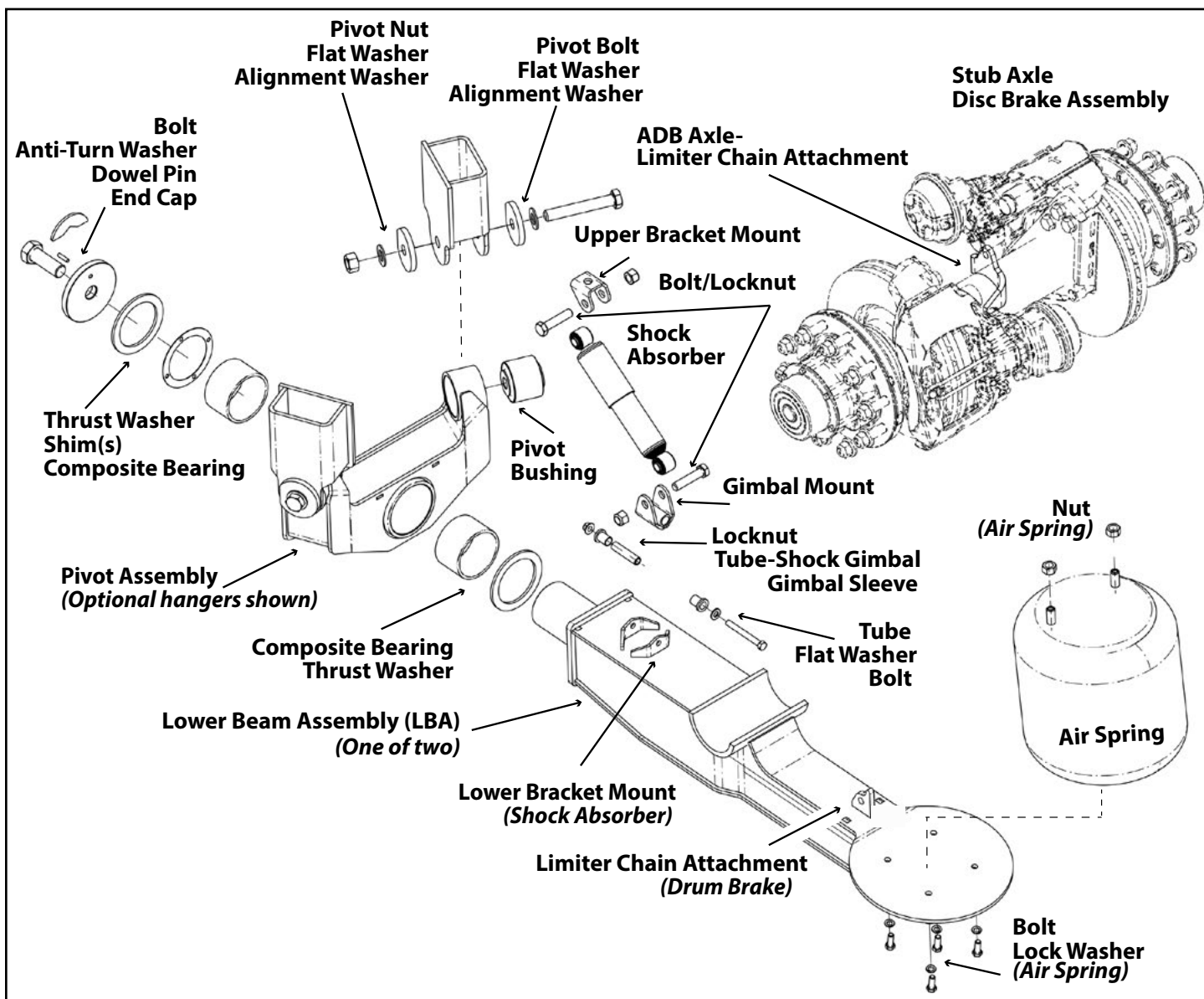
Figure 5. RAR-251 Stub-Axle Trailer Suspension (ADB assembly shown). Refer to the suspension model engineering drawing for the individual component part number.
