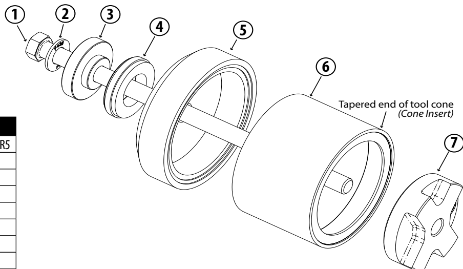
Figure 3. Tapered cone expands/compresses bushing for removal and installation.
