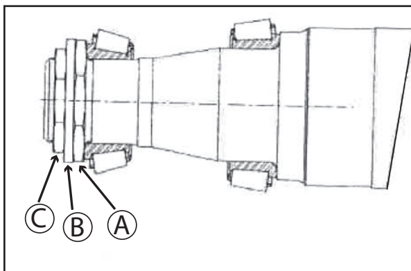
Figure 5. Double Adjusting Nut System
