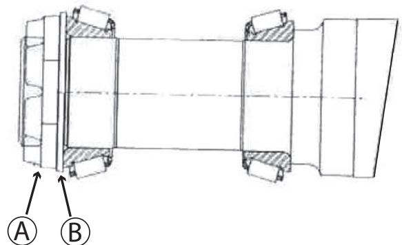
Figure 6. Single Adjusting Nut System
