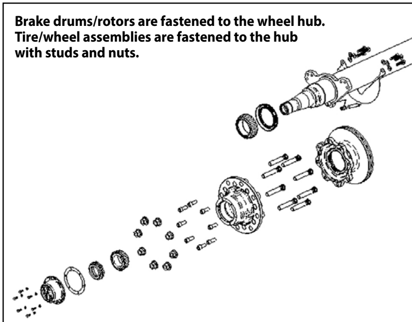
Figure 5. Wheel-End Equipment: Rotating components on the axle end such as the wheel hub; wheel bearings; the hub seal; the hubcap; and, related equipment such as tire inflation systems are listed as wheel-end equipment.
