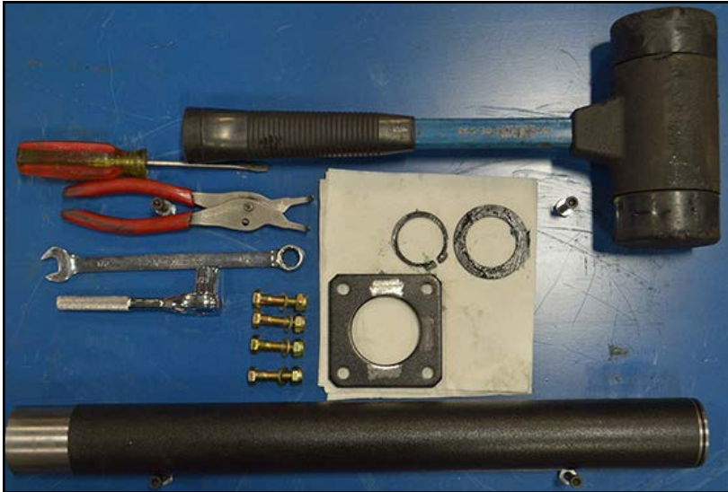
Drum Brake Axle - Cam Cover Service Kit includes the brake cam enclosure, the brake cam support bracket and hardware components for one cam cover replacement.
